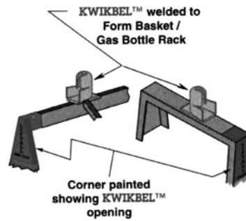
Painted corner showing Kwikbel™ opening
